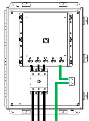
3-Phase DELTA, 3-Wire + Ground STZ240D...1
