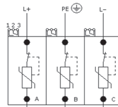
3 Pole - Photovoltaic
