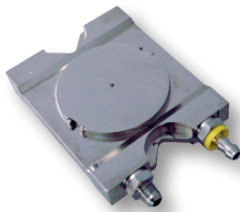
COLD PLATE FOR IGBT STACKS
