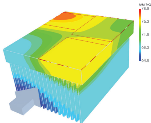
Air cooling simulation
